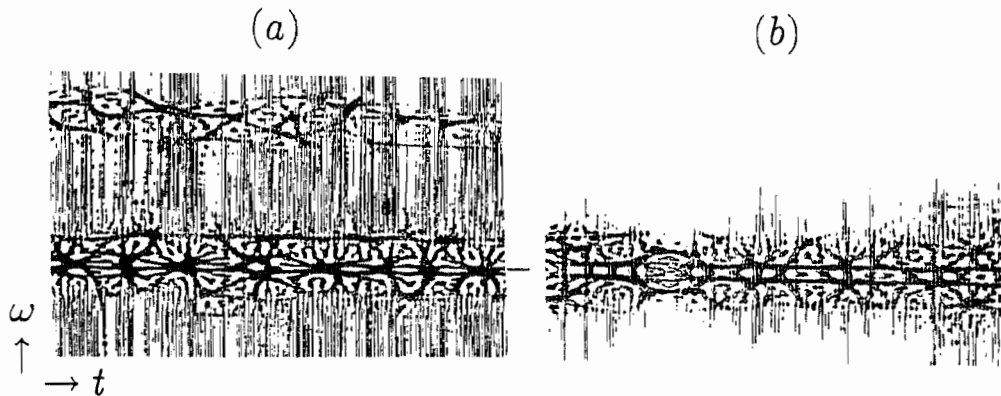
Fig. 5.9 Time-frequency plots of two car door slams. The one in (a) is characterized by a tinny sound and the one in (b) by a rich sound. The tinny sound is caused by the generation of a wide spectrum of frequencies in the initial contact of the door with the latch. (Courtesy of J. Feng, Ford Motor Co.)
