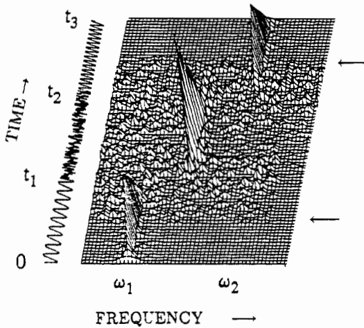
Fig. 8.7 The Wigner distribution is "noisy" because we have cross terms between the noise and between the noise and signal. Note that noise appears at times when there is no noise in the signal.
