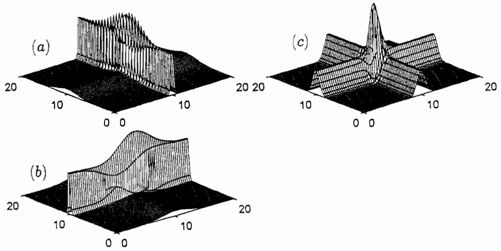
Fig. 7.1 Spectrograms of a signal composed of a constant frequency plus an impulse, s(t) = e^{j10t} + \delta(t-10) . In (a) we use a short duration window, which gives a good indication of when the impulse occurred but gives a broad localization for the frequency. In (b) we use a long duration window, which gives the opposite effect. In (c) a compromise window is used. For a comparison with the Wigner distribution see Fig. 8.5.
