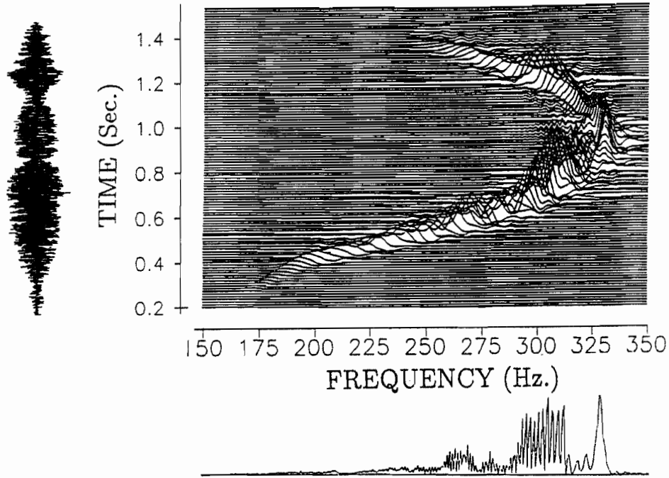
Fig. 5.1 A time-frequency plot of a sound made by a Bowhead whale. The wave form is on the left plot with time increasing upwards. The energy density spectrum is below the main figure and indicates which frequencies existed for the duration. The main figure is a joint time-frequency plot and shows how the frequencies change with time. (From the work of C. Rosenthal and L. Cohen.)
