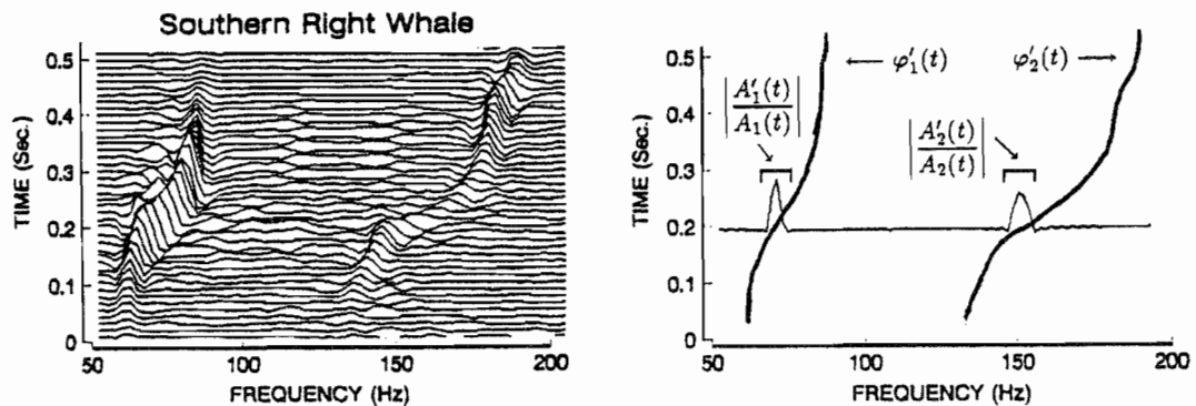
Fig. 13.2 A multicomponent signal is characterized by the narrowness of both parts in comparison to their separation.
