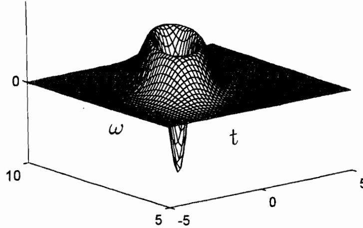
Fig. 8.4 The Wigner distribution for the signal s(t) = t e^{-\alpha t^2/2 + j\beta t^2/2 + j\omega_0 t} . Everything below the plane is negative.
