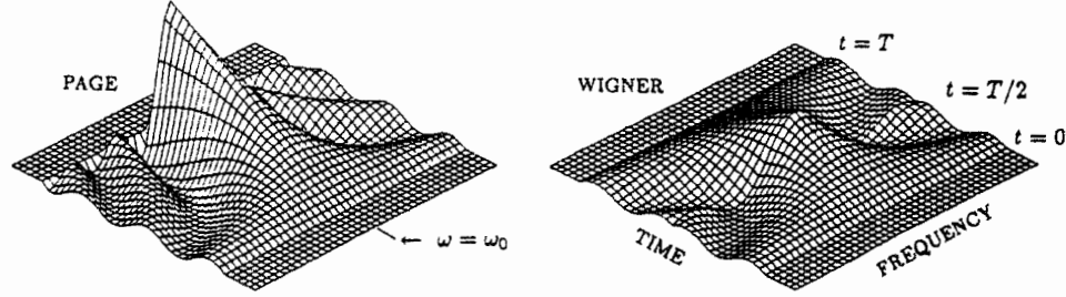
Fig. 12.9 A comparison of the Wigner distribution and Page distribution for a finite duration sine wave. The Page distribution does not go to zero at the end of the signal.
